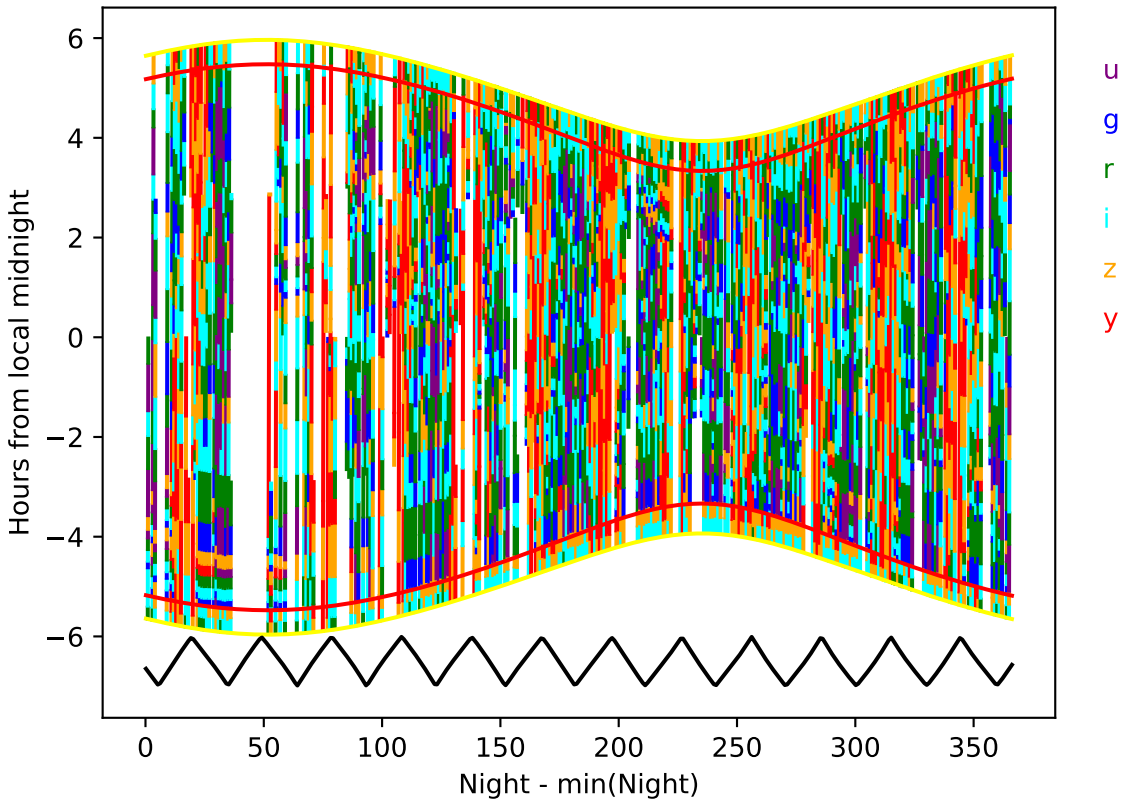
internal_u_expt60_nscale1.0v3.4_10yrs year 2-3: Hourglass
