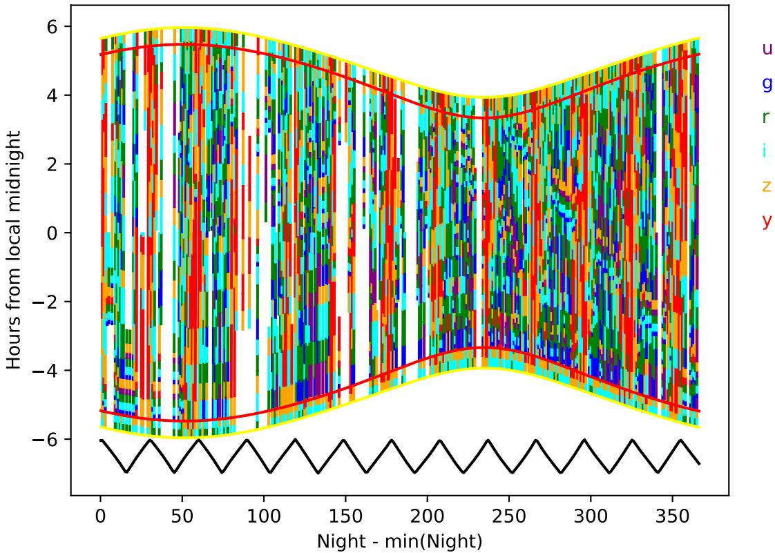
internal_u_expt60_nscale1.0v3.4_10yrs year 1-2: Hourglass
