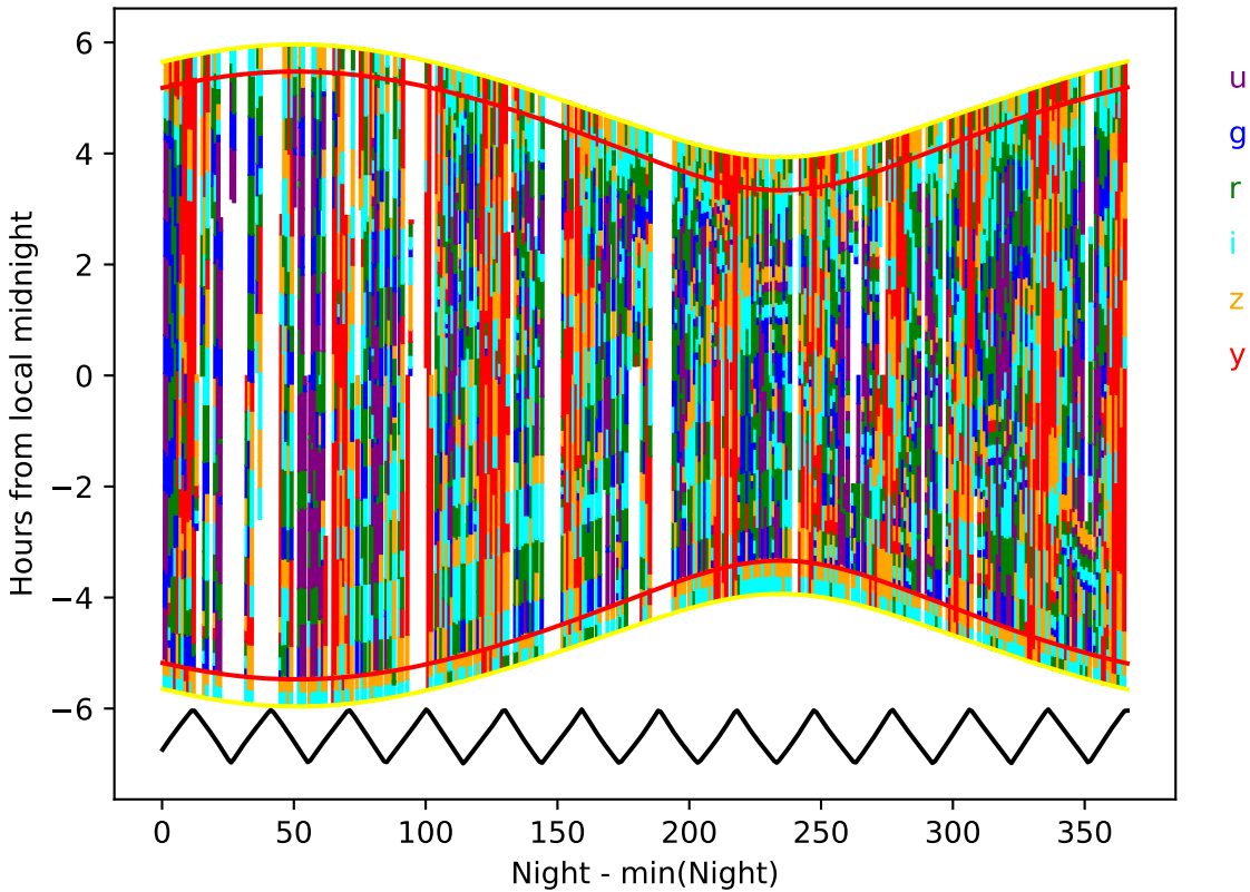
internal_u_expt60_nscale1.0v3.4_10yrs year 0-1: Hourglass
