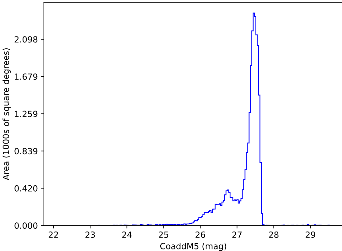
internal_u_expt60_nscale1.0v3.4_10yrs : CoaddM5
