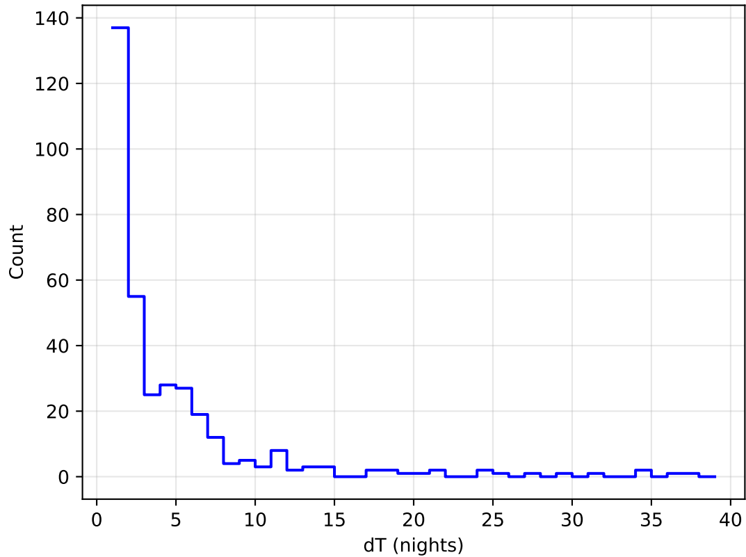
internal_u_expt60_nscale1.0v3.4_10yrs all bands: DD:WFD Delta Nights Histogram
