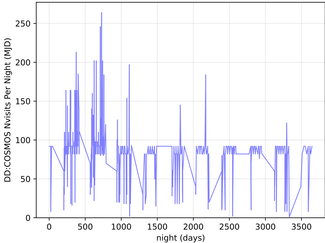
internal_u_expt60_nscale1.0v3.4_10yrs all bands: DD: COSMOS Nvisits Per Night
