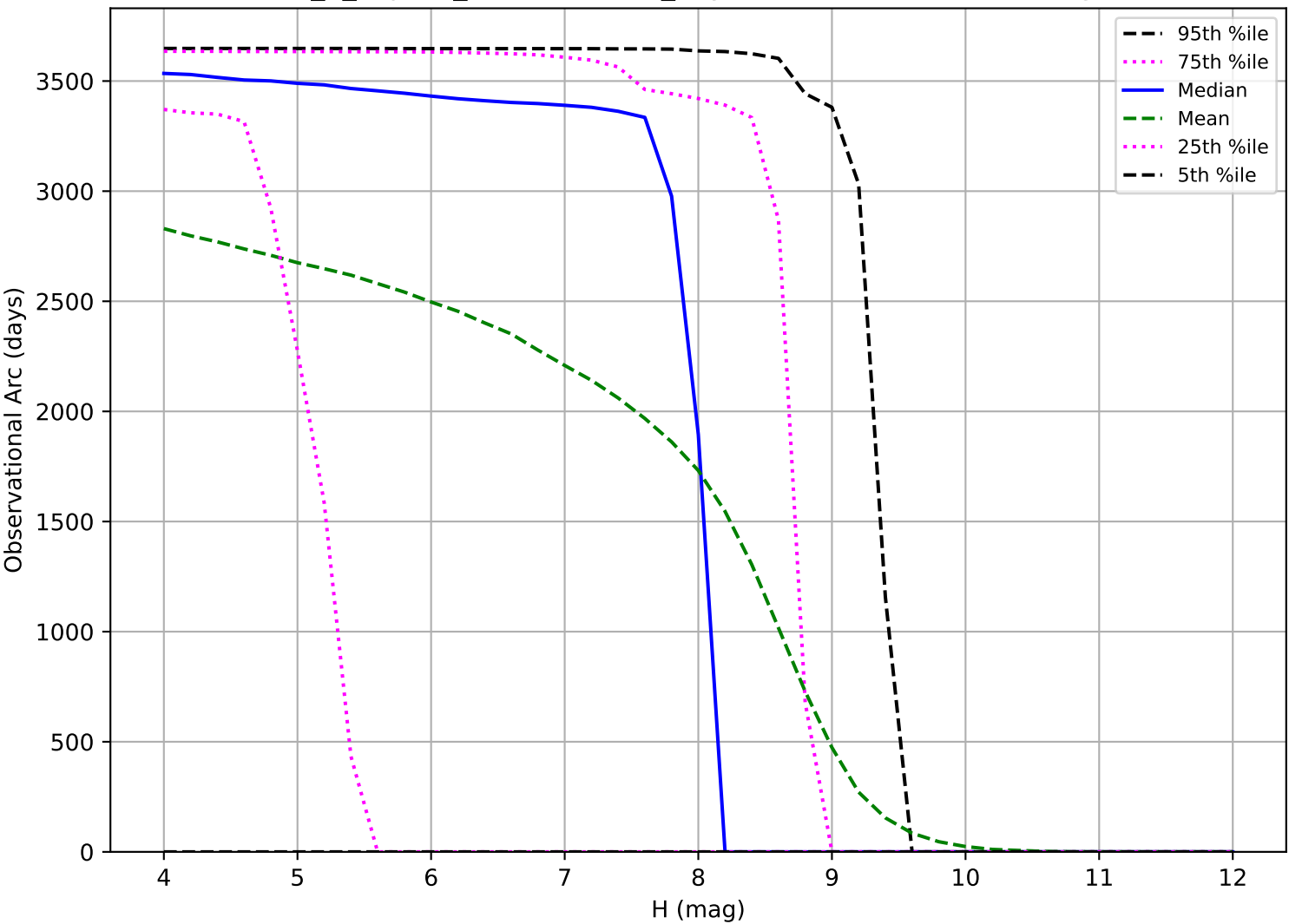
internal_u_expt60_nscale0.9v3.4_10yrs: Observational Arc Length TNO
