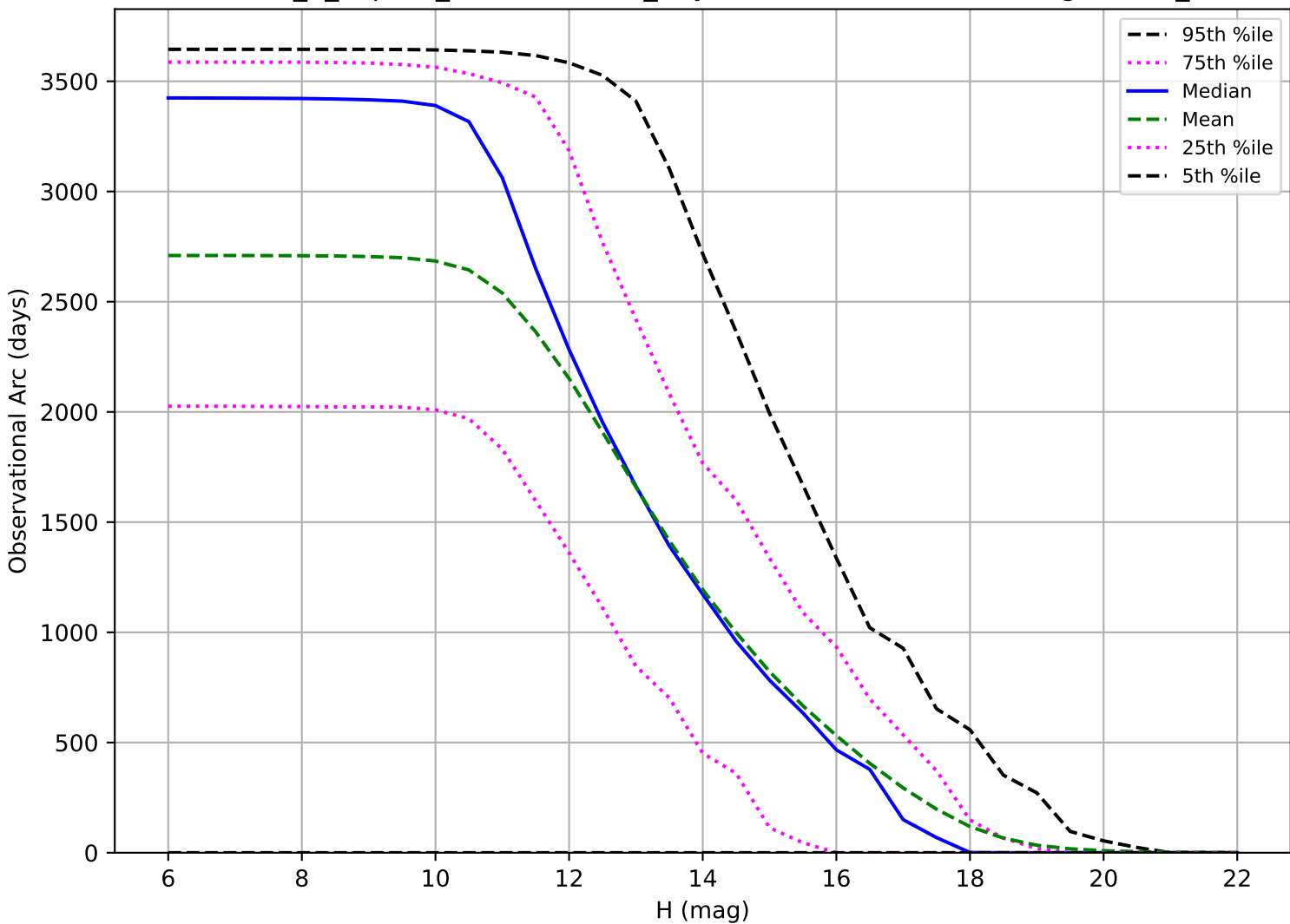
internal_u_expt60_nscale0.9v3.4_10yrs: Observational Arc Length OCC_r5
