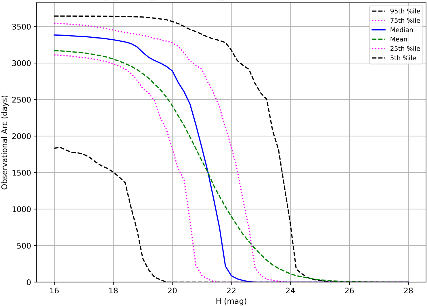
internal_u_expt60_nscale0.9v3.4_10yrs: Observational Arc Length NEO
