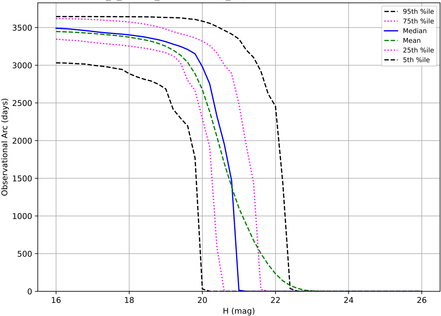
internal_u_expt60_nscale0.9v3.4_10yrs: Observational Arc Length MBA
