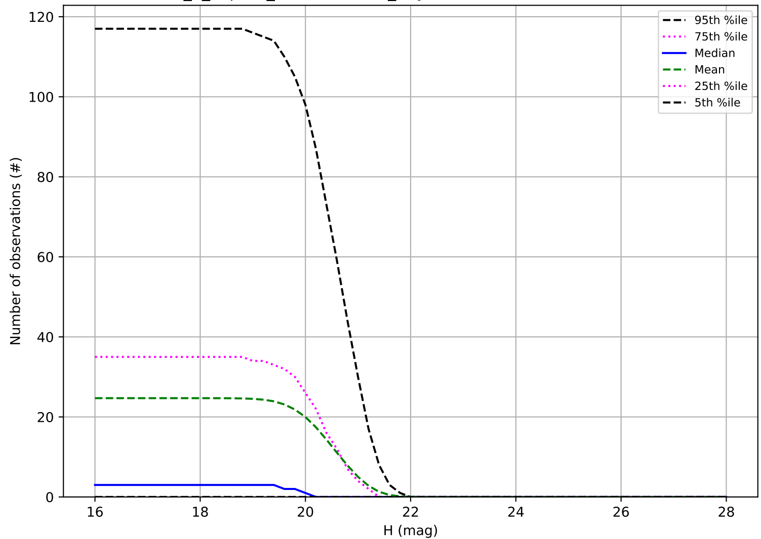
internal_u_expt60_nscale0.9v3.4_10yrs: Number of observations Vatira
