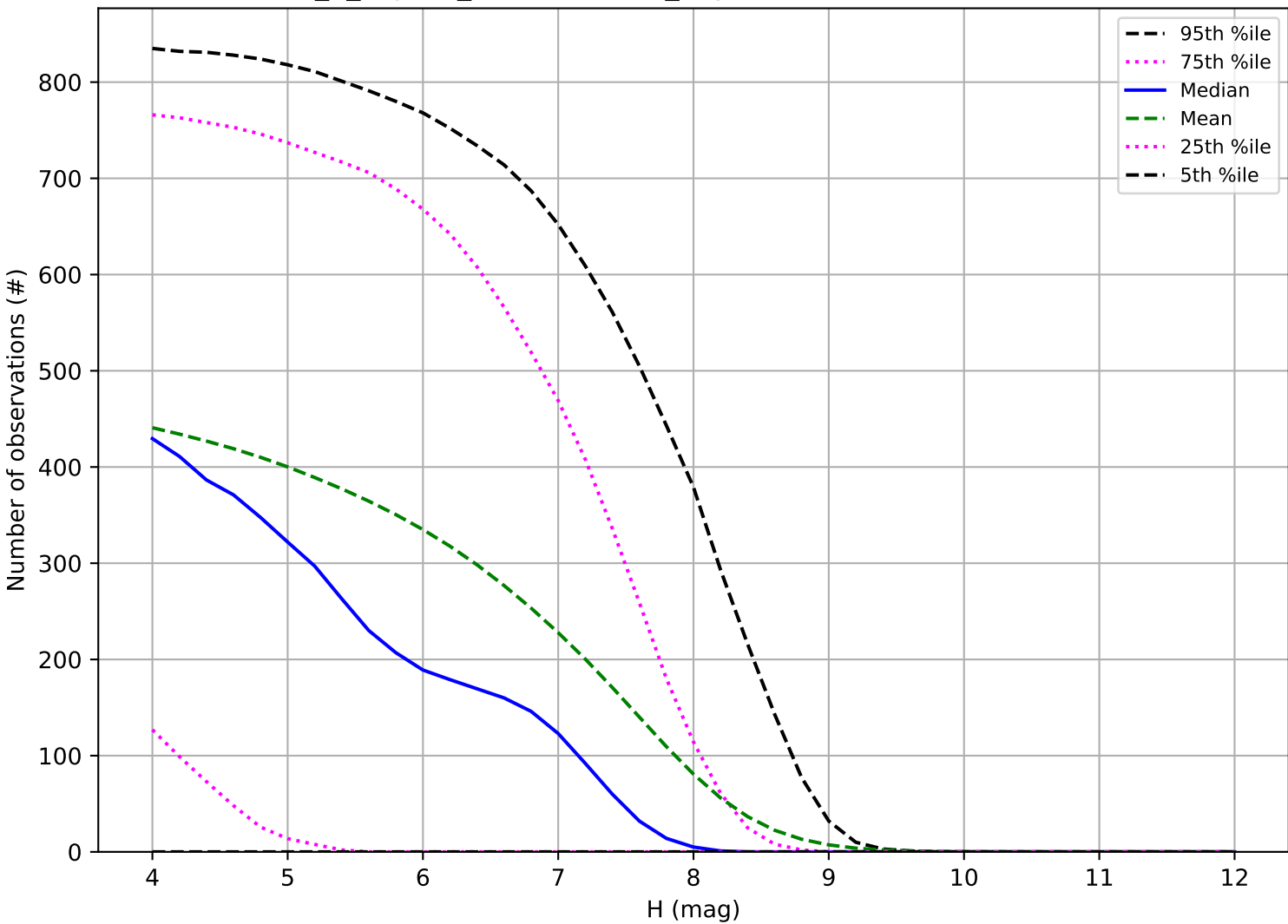
internal_u_expt60_nscale0.9v3.4_10yrs: Number of observations TNO
