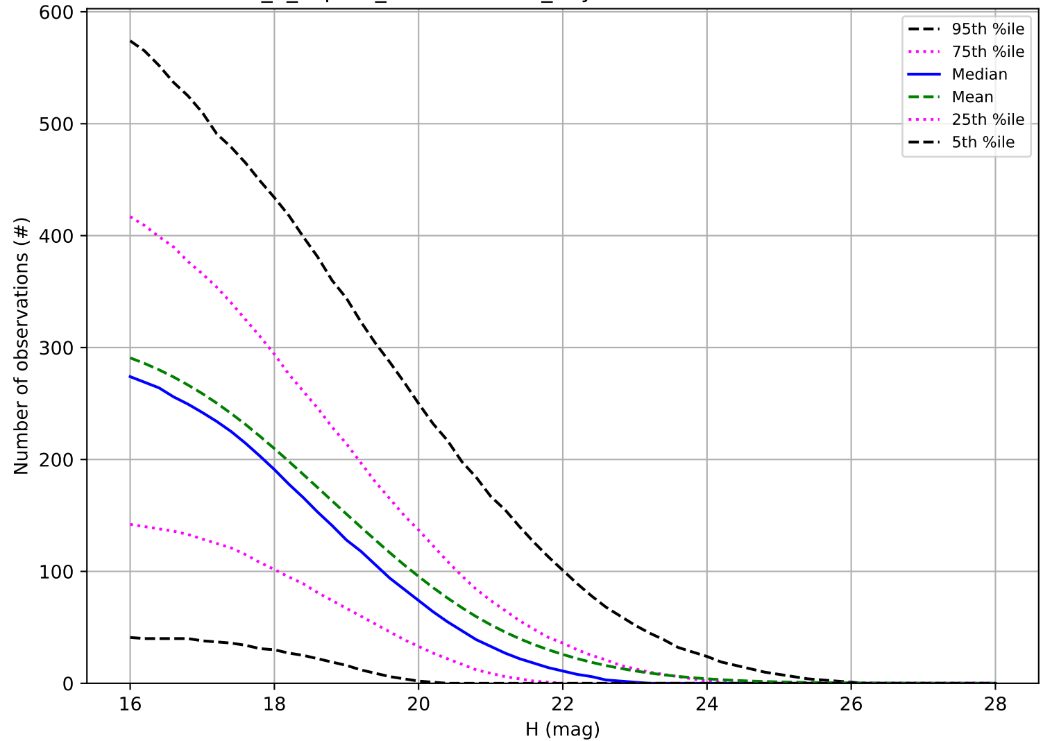
internal_u_expt60_nscale0.9v3.4_10yrs: Number of observations PHA
