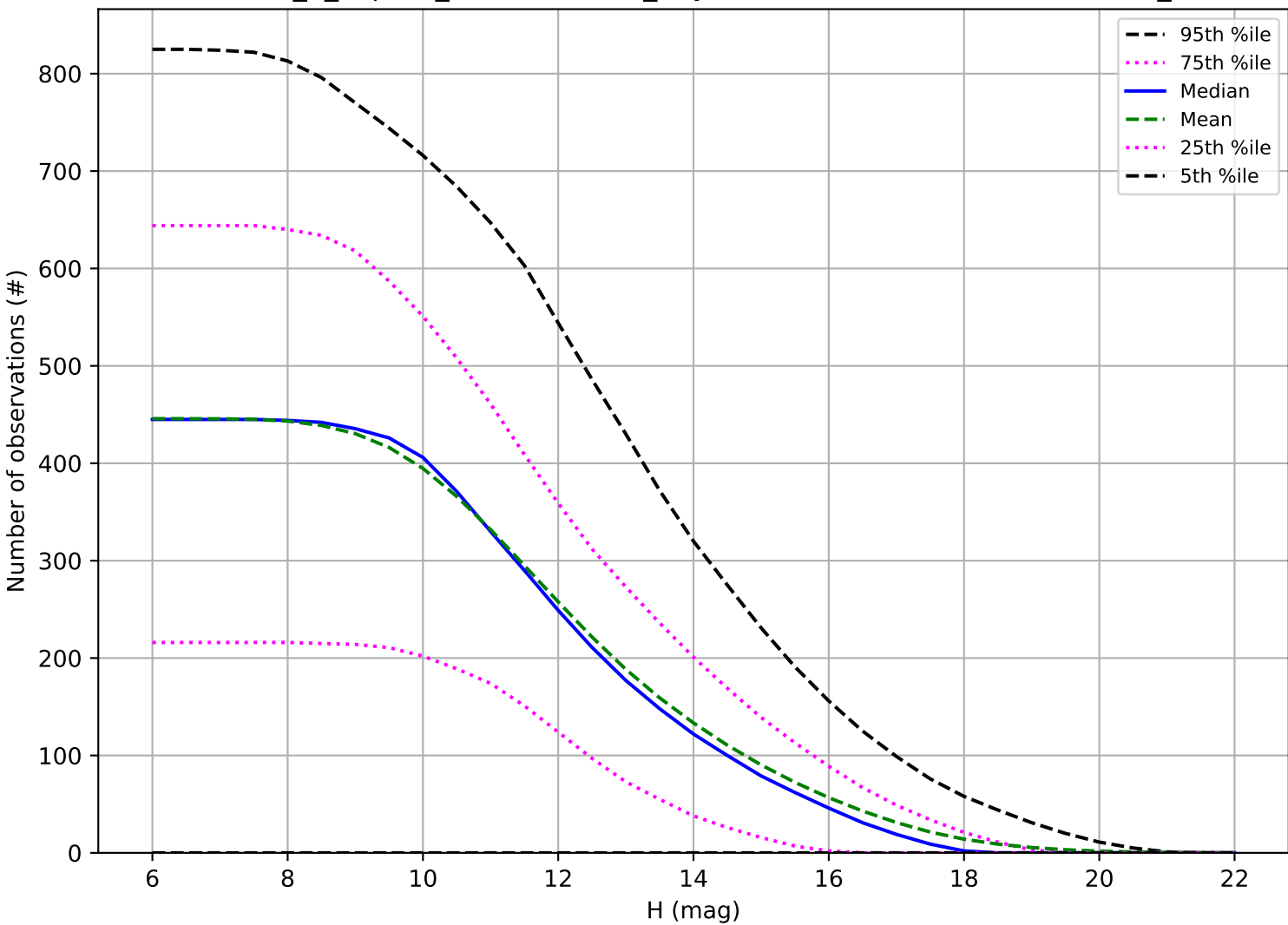
internal_u_expt60_nscale0.9v3.4_10yrs: Number of observations OCC_r5
