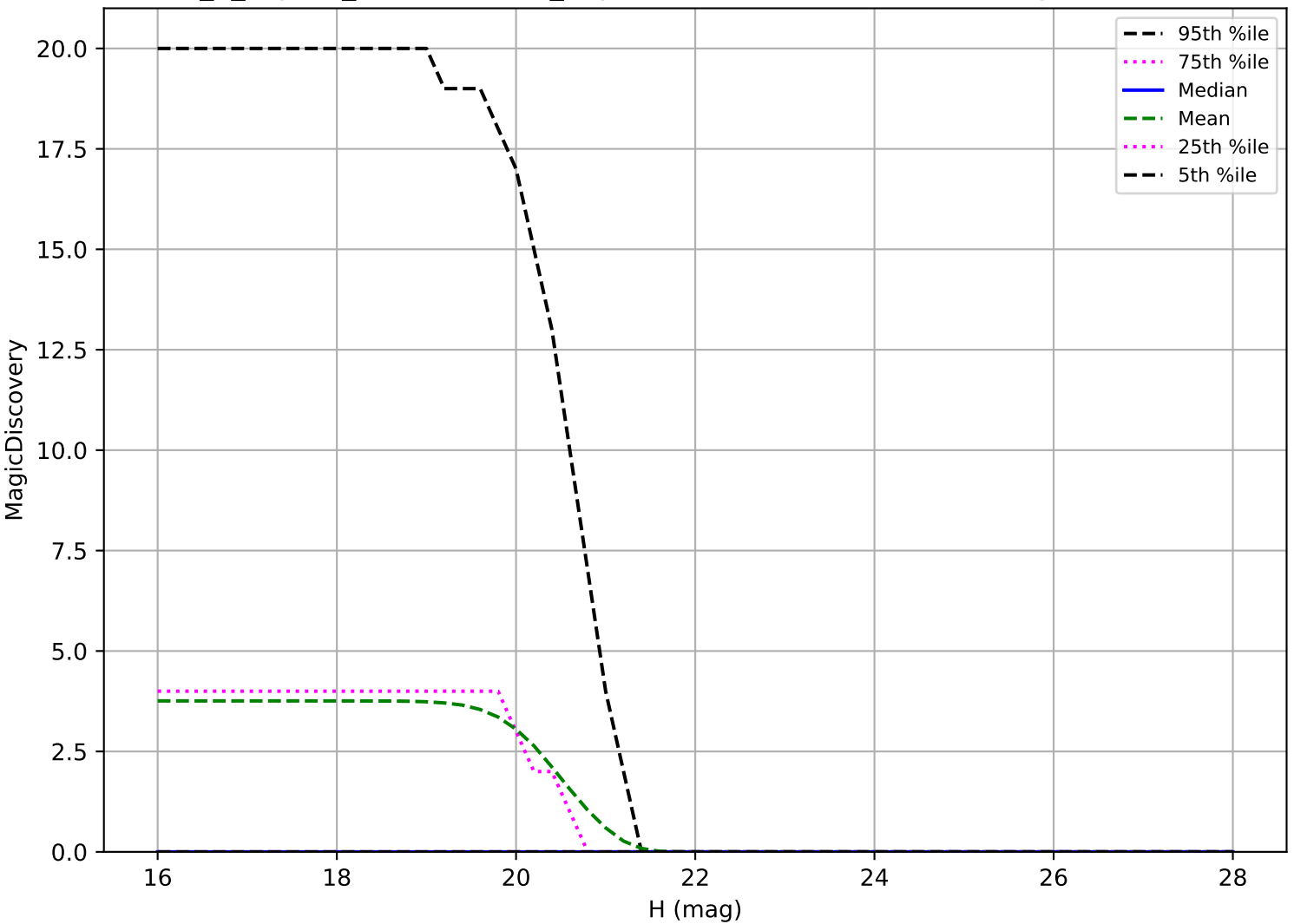
internal_u_expt60_nscale0.9v3.4_10yrs: Vatira 6 detections in 60 nights detection loss
