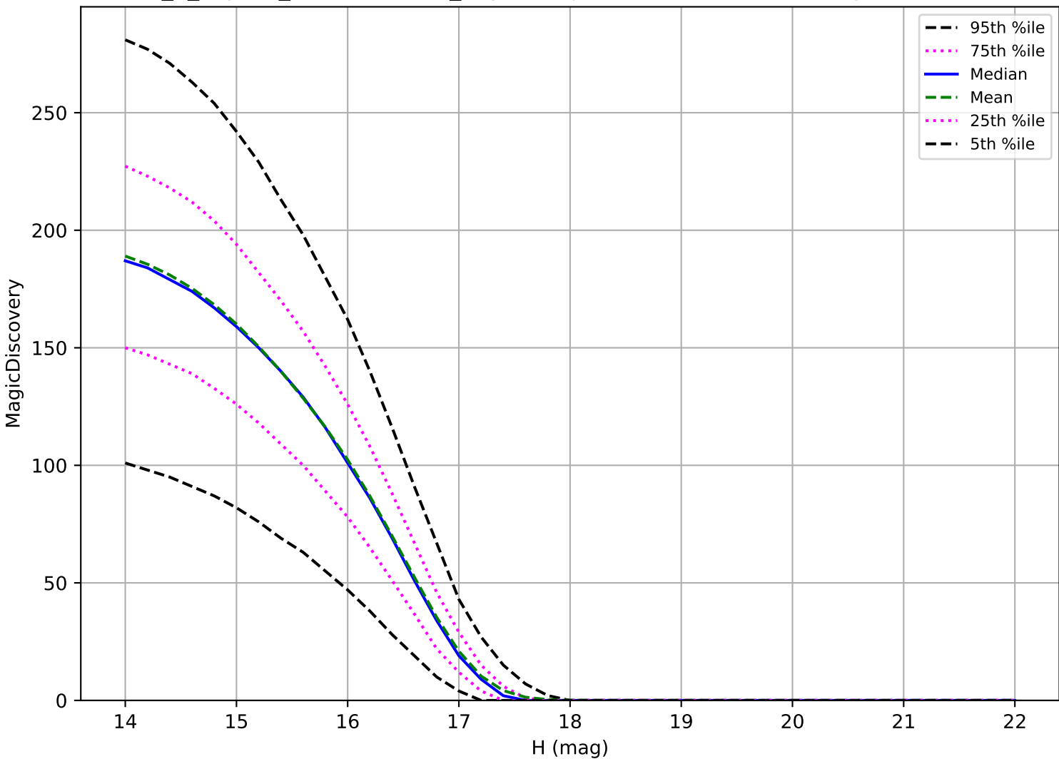
internal_u_expt60_nscale0.9v3.4_10yrs: Trojan 6 detections in 60 nights detection loss
