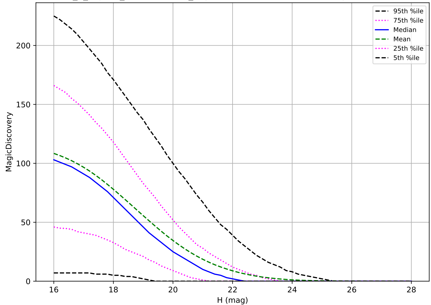
internal_u_expt60_nscale0.9v3.4_10yrs: PHA 6 detections in 60 nights detection loss
