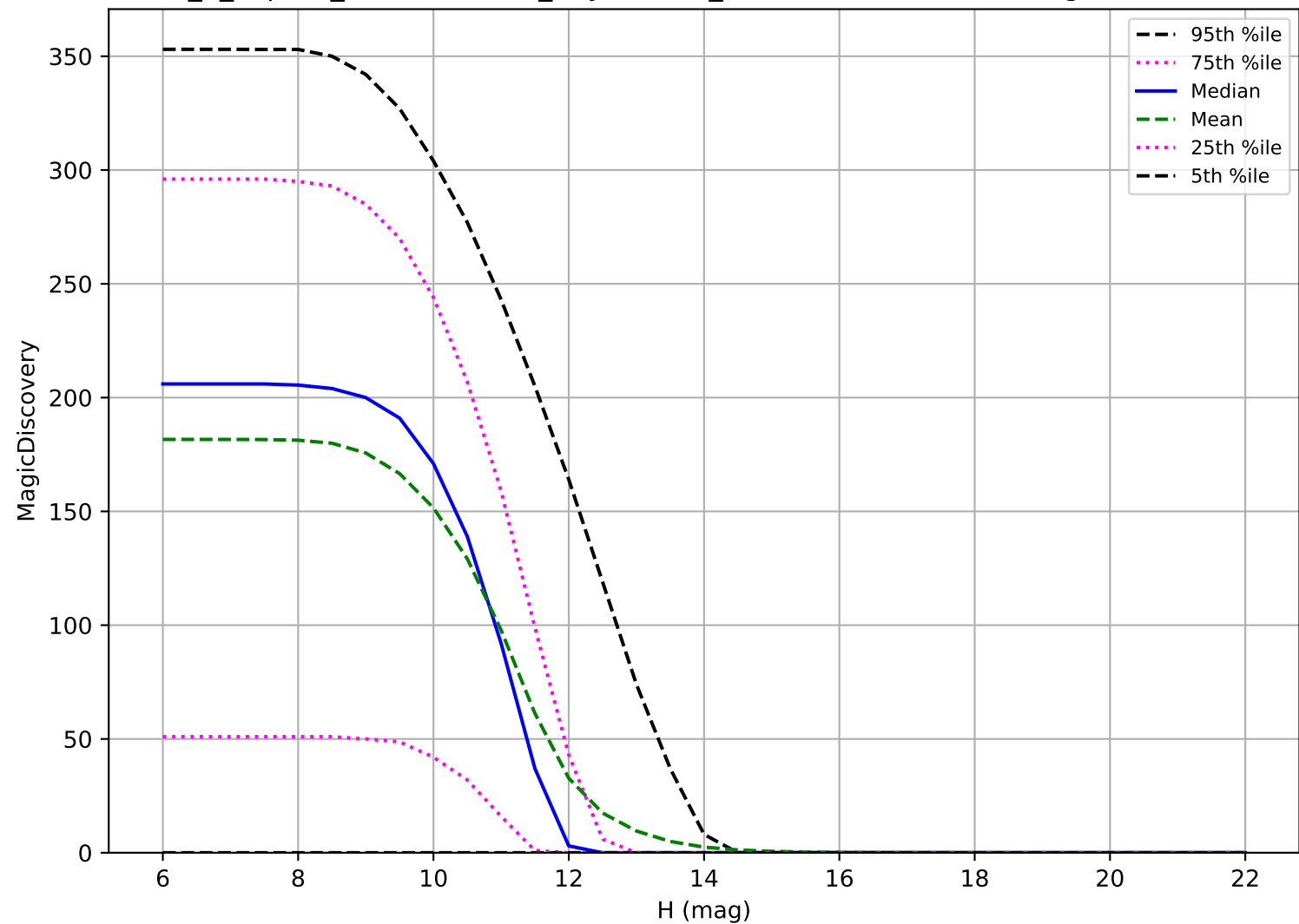
internal_u_expt60_nscale0.9v3.4_10yrs: OCC_r20 6 detections in 60 nights detection loss
