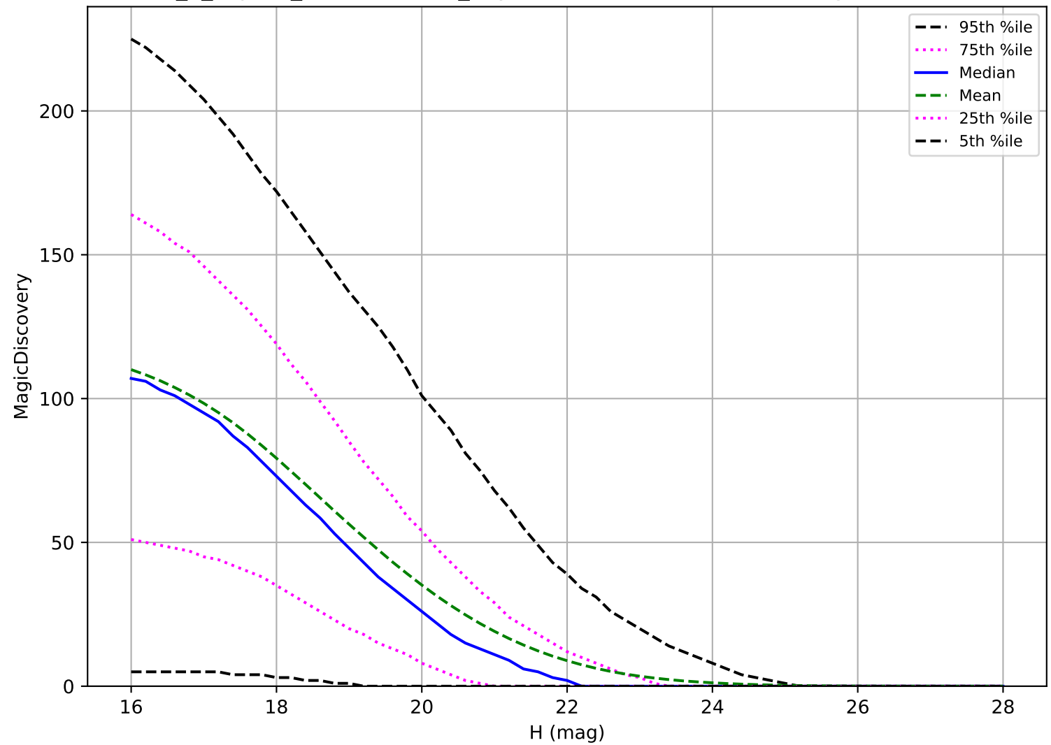
internal_u_expt60_nscale0.9v3.4_10yrs: NEO 6 detections in 60 nights detection loss
