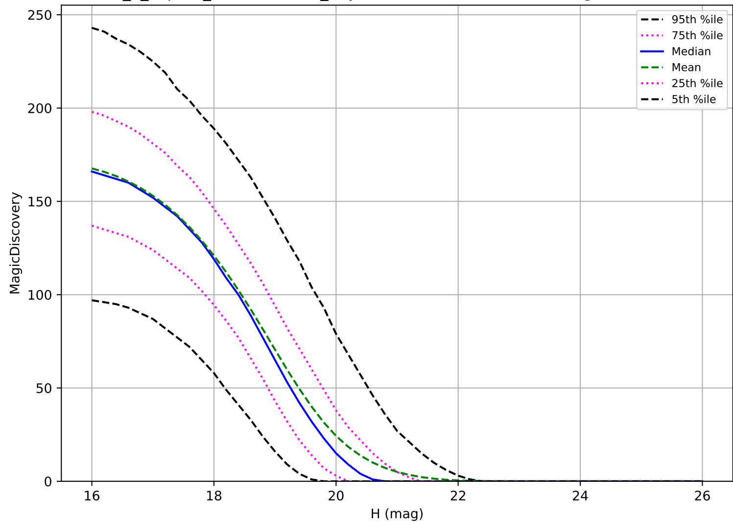
internal_u_expt60_nscale0.9v3.4_10yrs: MBA 6 detections in 60 nights detection loss
