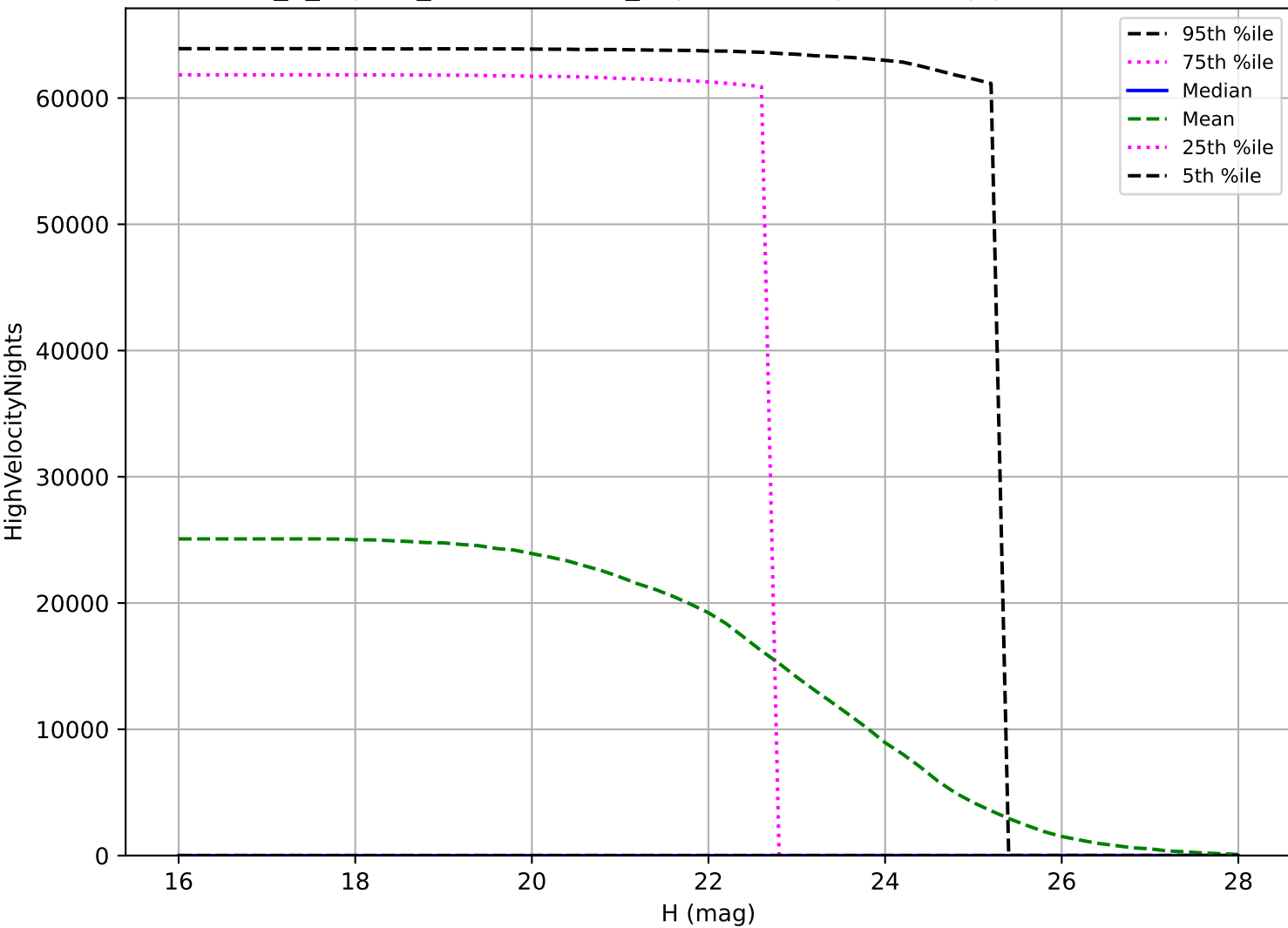
internal_u_expt60_nscale0.9v3.4_10yrs: PHA High velocity pair detection loss
