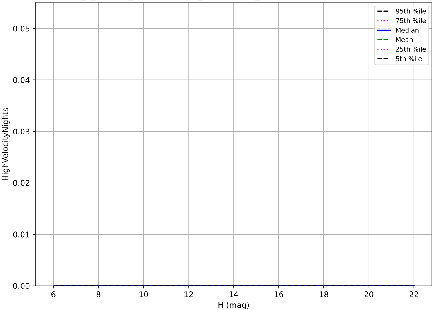
internal_u_expt60_nscale0.9v3.4_10yrs: OCC_r5 High velocity pair detection loss
