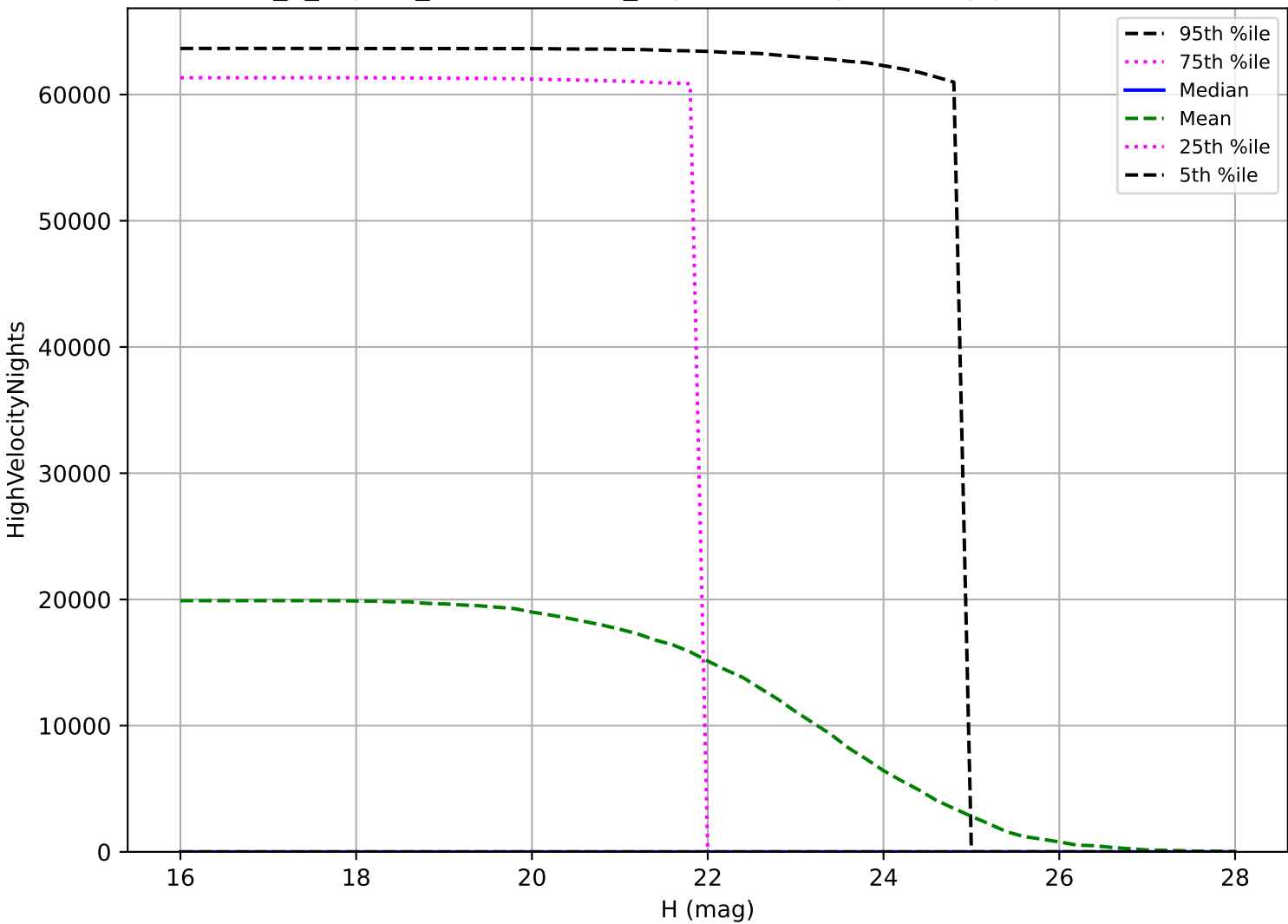
internal_u_expt60_nscale0.9v3.4_10yrs: NEO High velocity pair detection loss
