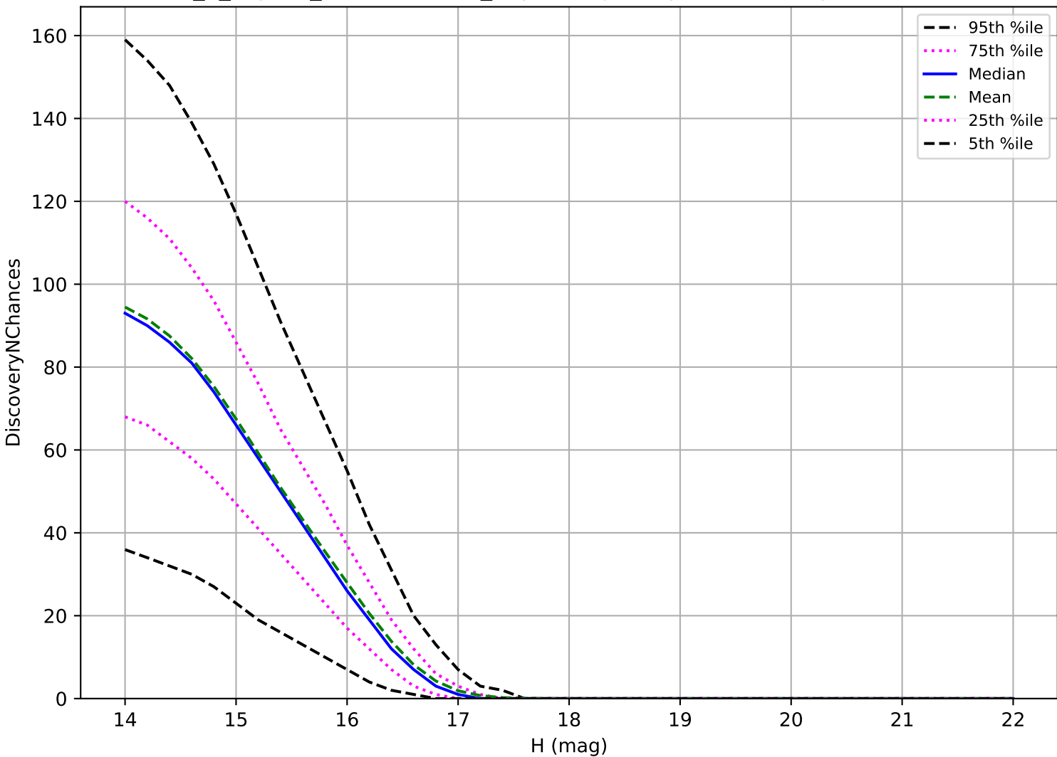
internal_u_expt60_nscale0.9v3.4_10yrs: Trojan 3 pairs in 15 nights detection loss
