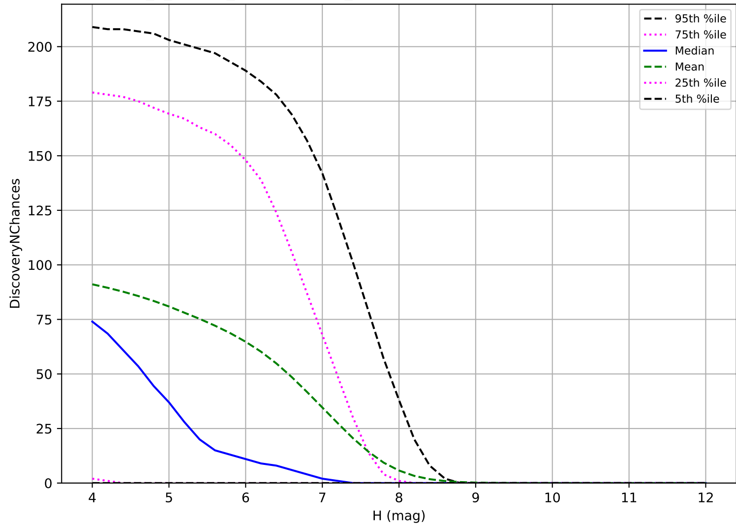
internal_u_expt60_nscale0.9v3.4_10yrs: TNO 3 pairs in 15 nights detection loss
