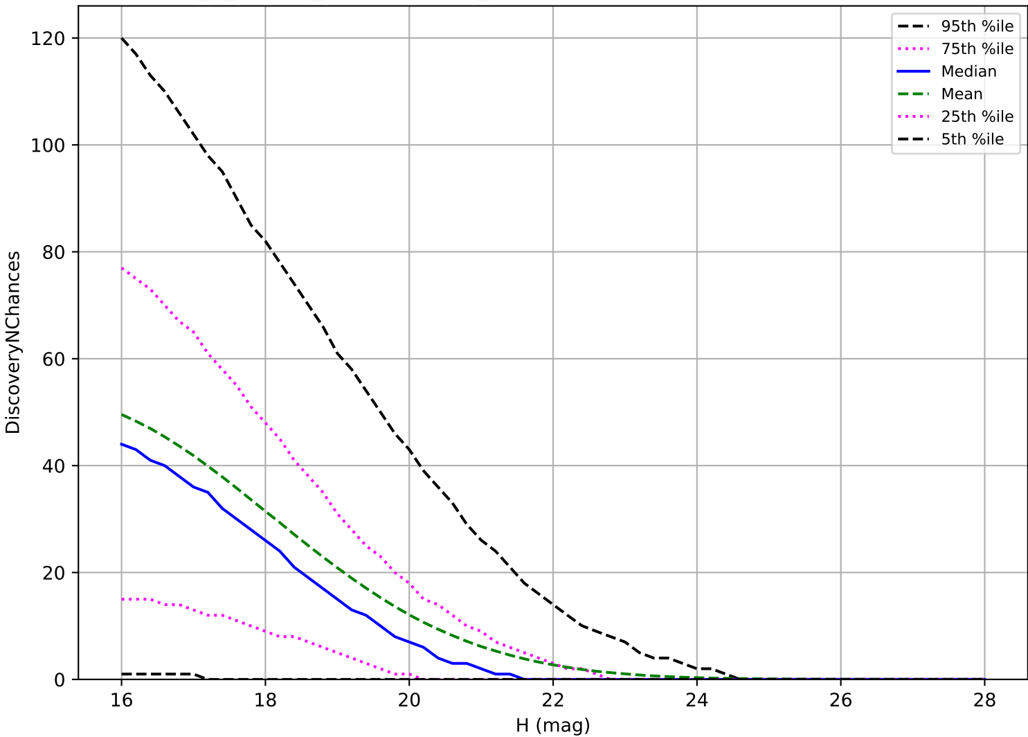
internal_u_expt60_nscale0.9v3.4_10yrs: PHA 3 pairs in 15 nights detection loss
