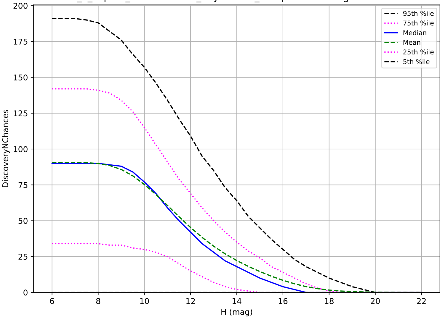
internal_u_expt60_nscale0.9v3.4_10yrs: OCC_r5 3 pairs in 15 nights detection loss
