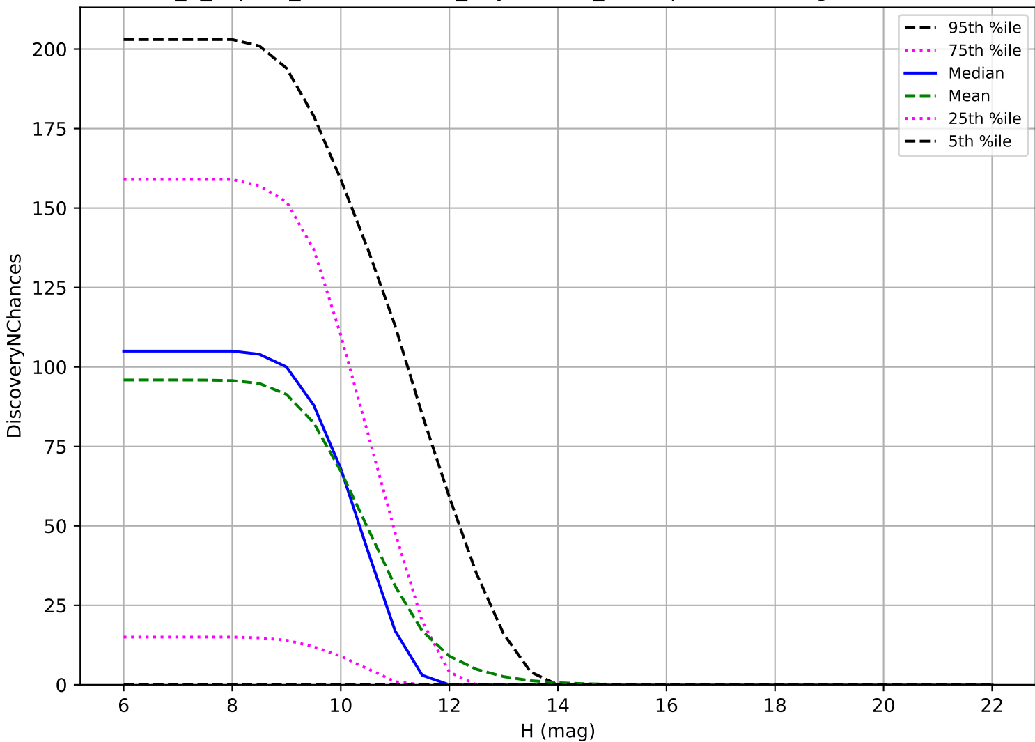
internal_u_expt60_nscale0.9v3.4_10yrs: OCC_r20 3 pairs in 15 nights detection loss
