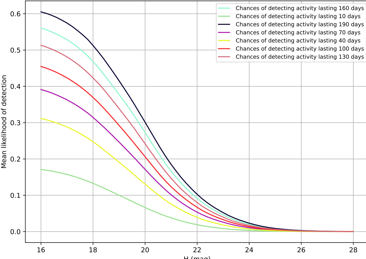
internal_u_expt60_nscale0.9v3.4_10yrs PHA
