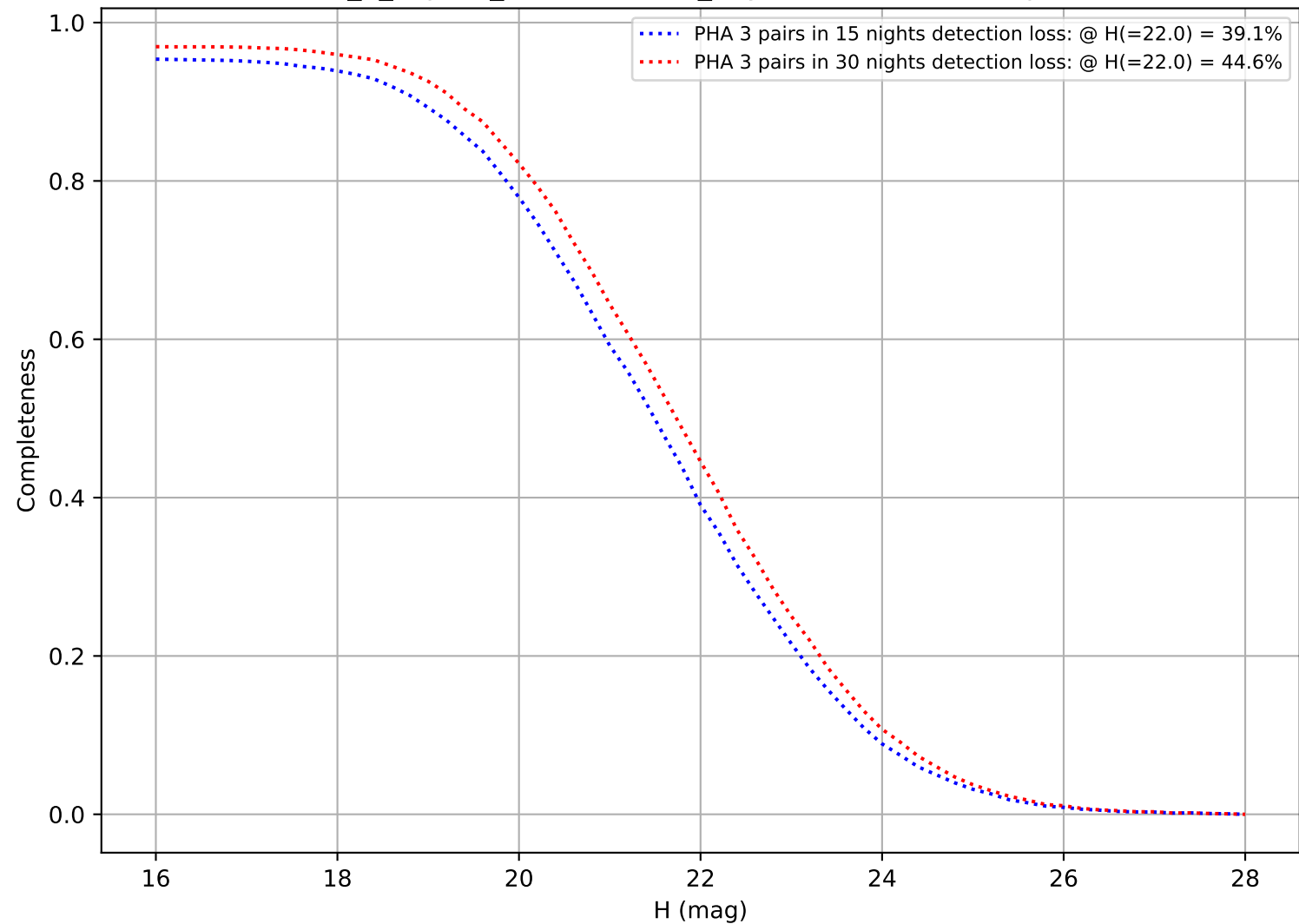
internal_u_expt60_nscale0.9v3.4_10yrs: DifferentialCompleteness
