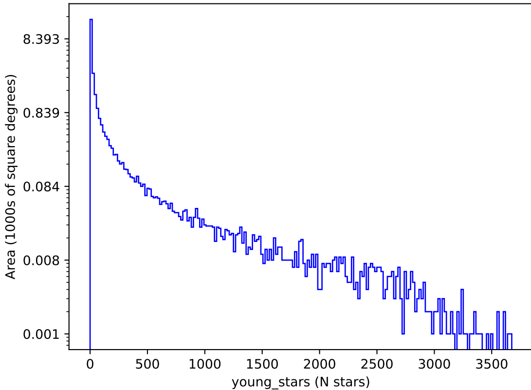
internal_u_expt60_nscale0.9v3.4_10yrs : young_stars
