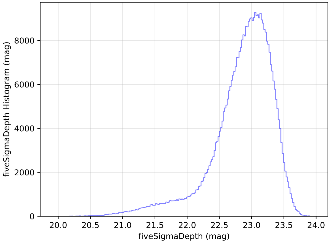
internal_u_expt60_nscale0.9v3.4_10yrs z: fiveSigmaDepth Histogram
