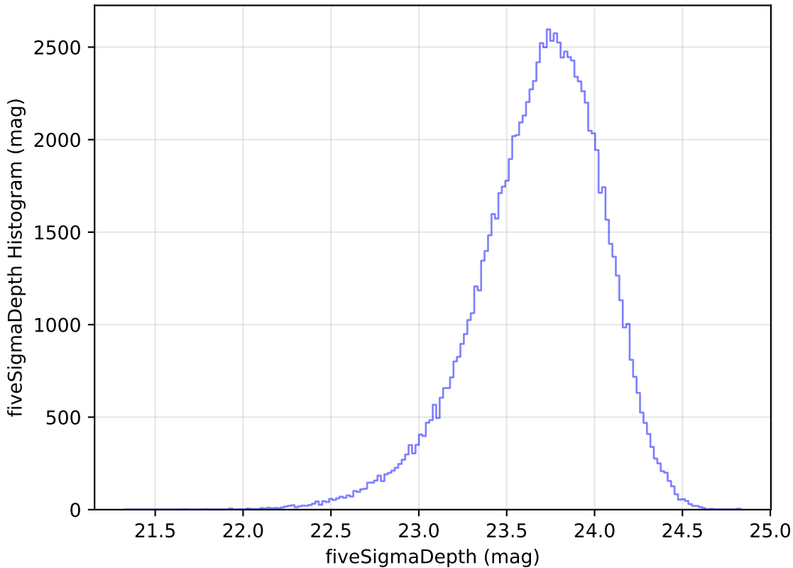
internal_u_expt60_nscale0.9v3.4_10yrs u: fiveSigmaDepth Histogram
