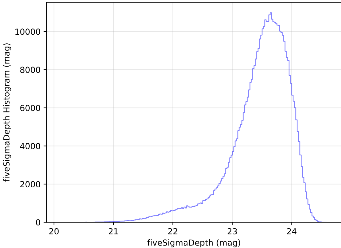
internal_u_expt60_nscale0.9v3.4_10yrs i: fiveSigmaDepth Histogram
