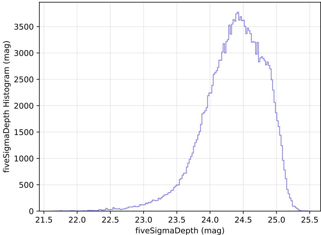
internal_u_expt60_nscale0.9v3.4_10yrs g: fiveSigmaDepth Histogram
