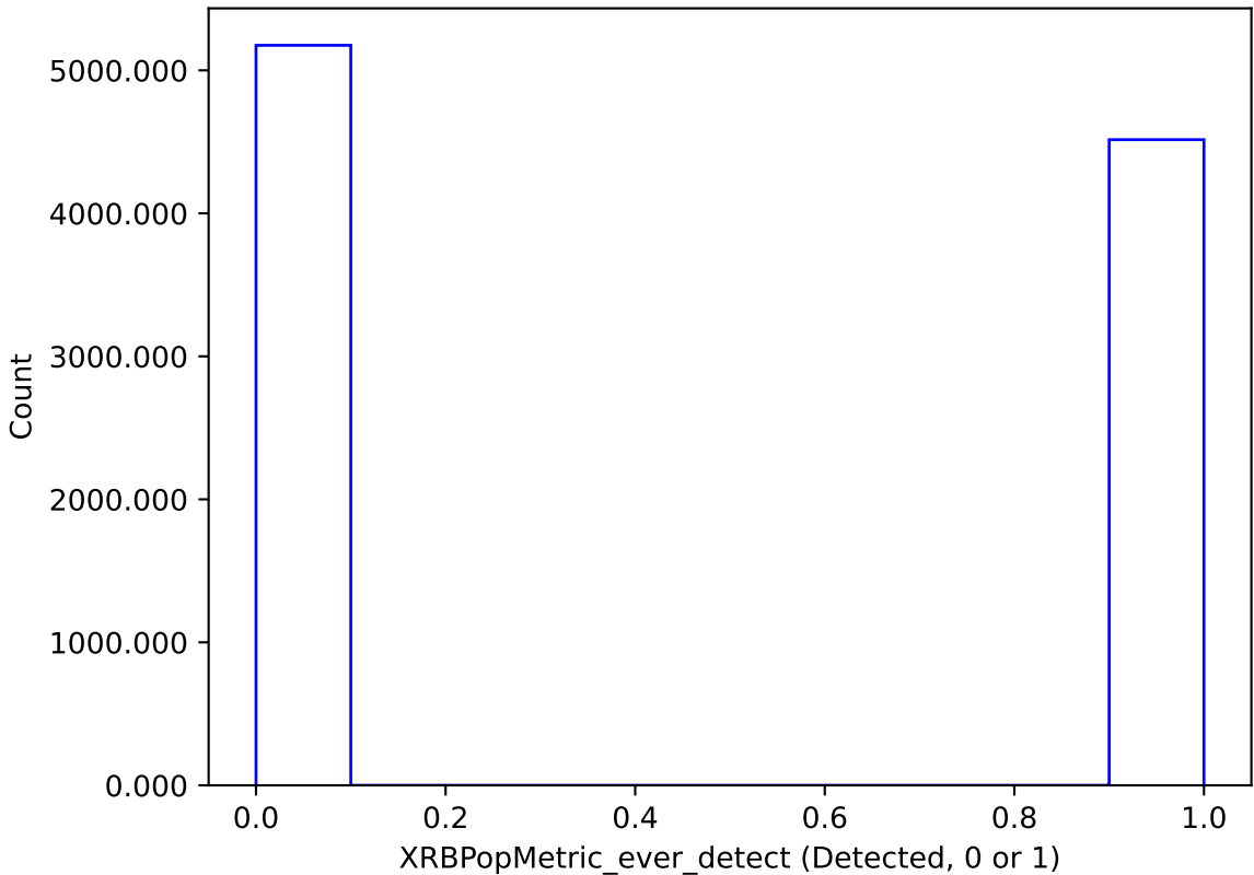
internal_u_expt60_nscale0.9v3.4_10yrs : XRBPoMetric_ever_detect
