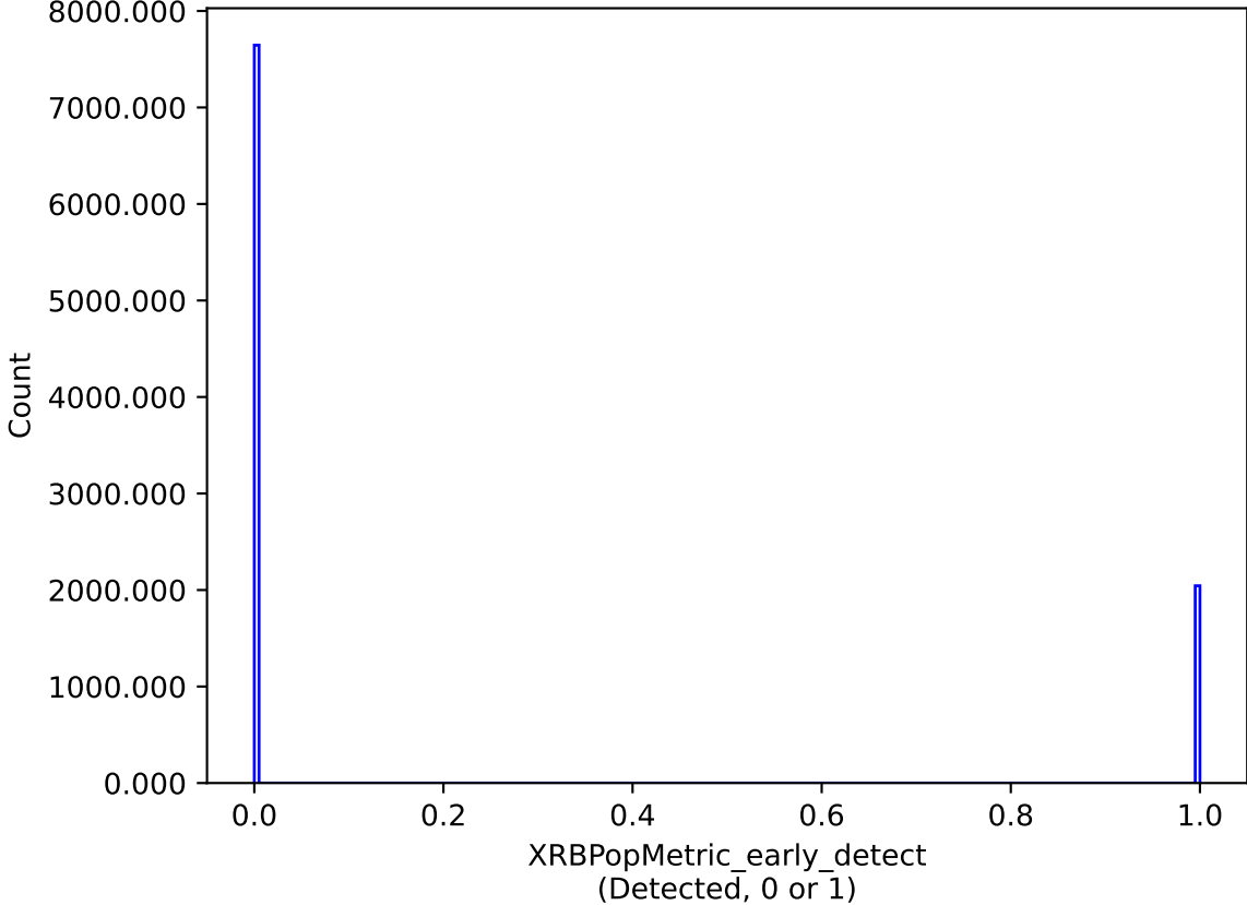
internal_u_expt60_nscale0.9v3.4_10yrs : XRBPoMetric_early_detect
