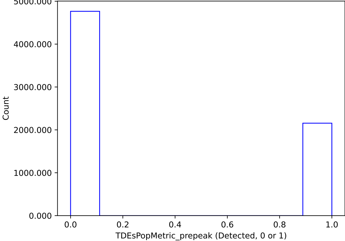
internal_u_expt60_nscale0.9v3.4_10yrs : TDEsPopMetric_prepeak
