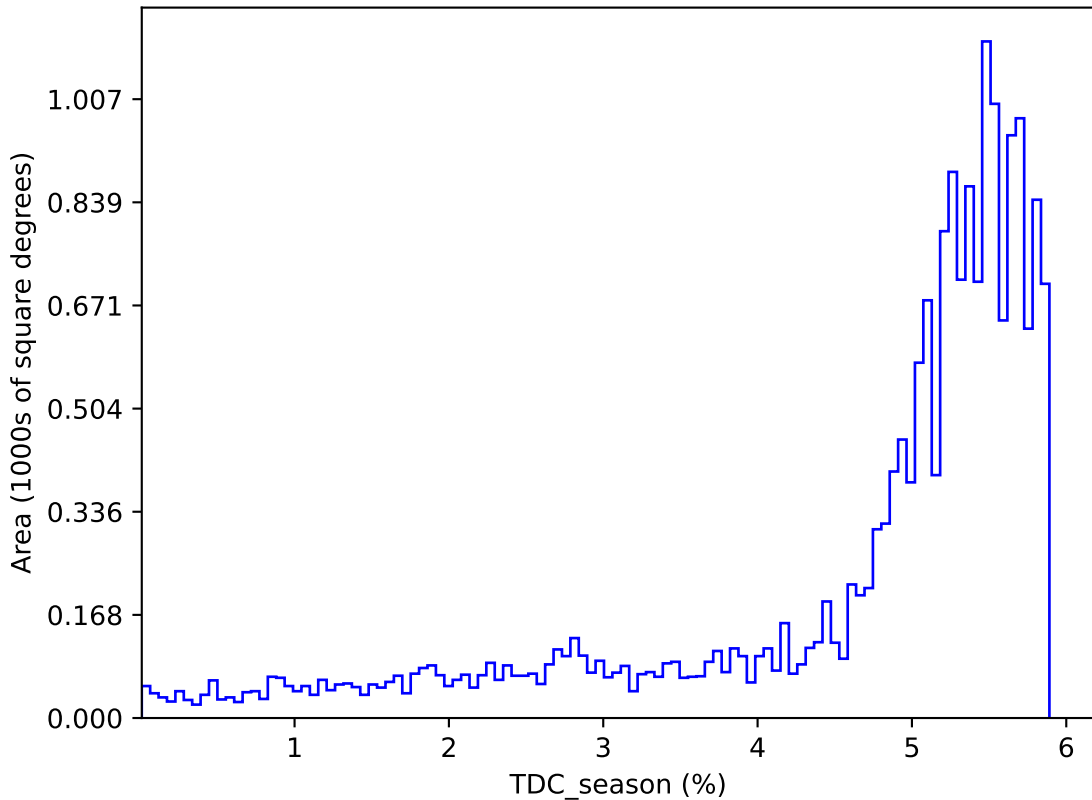
internal_u_expt60_nscale0.9v3.4_10yrs : TDC_season
