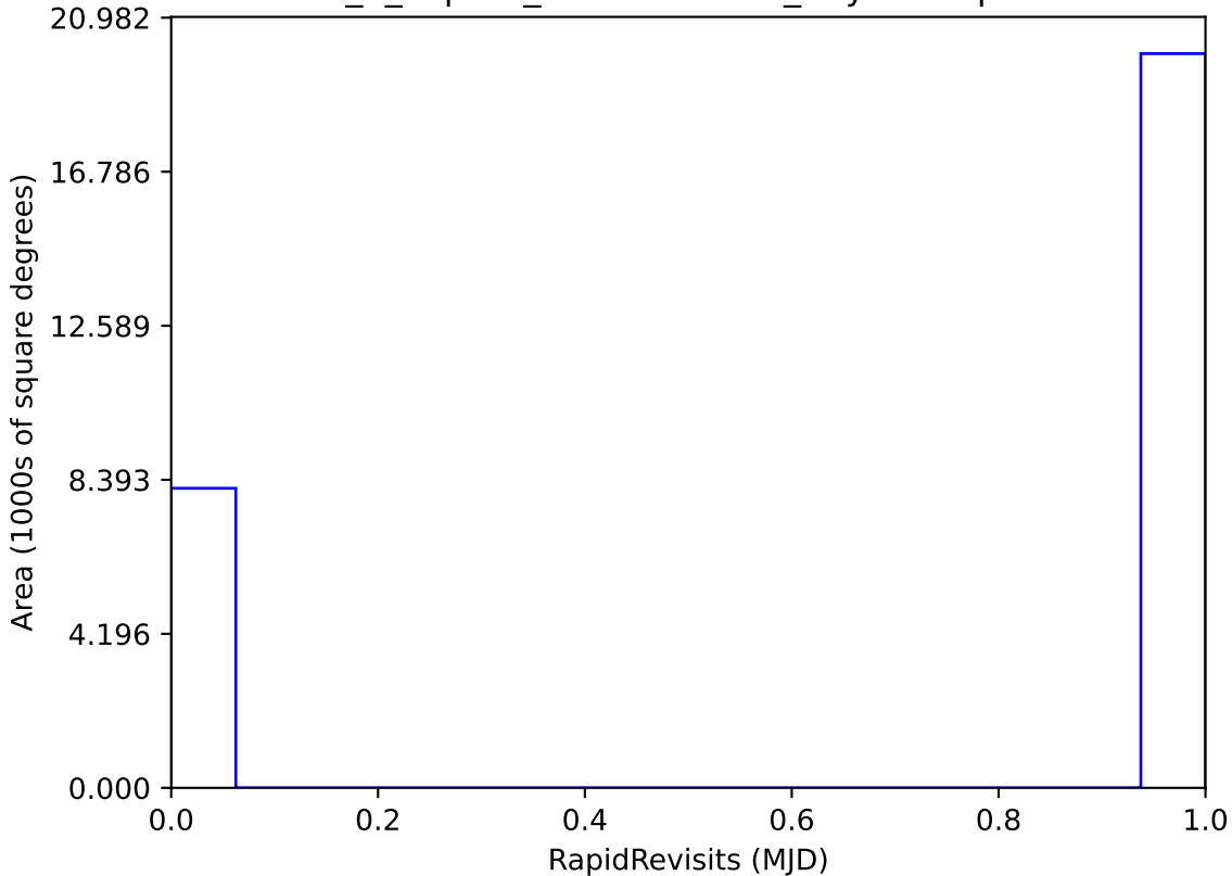
internal_u_expt60_nscale0.9v3.4_10yrs : RapidRevisits
