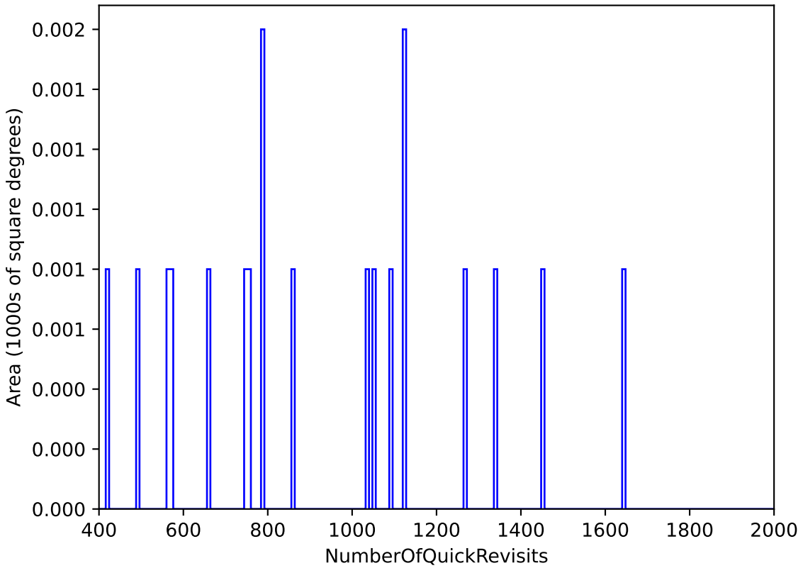
internal_u_expt60_nscale0.9v3.4_10yrs : NumberOfQuickRevisits
