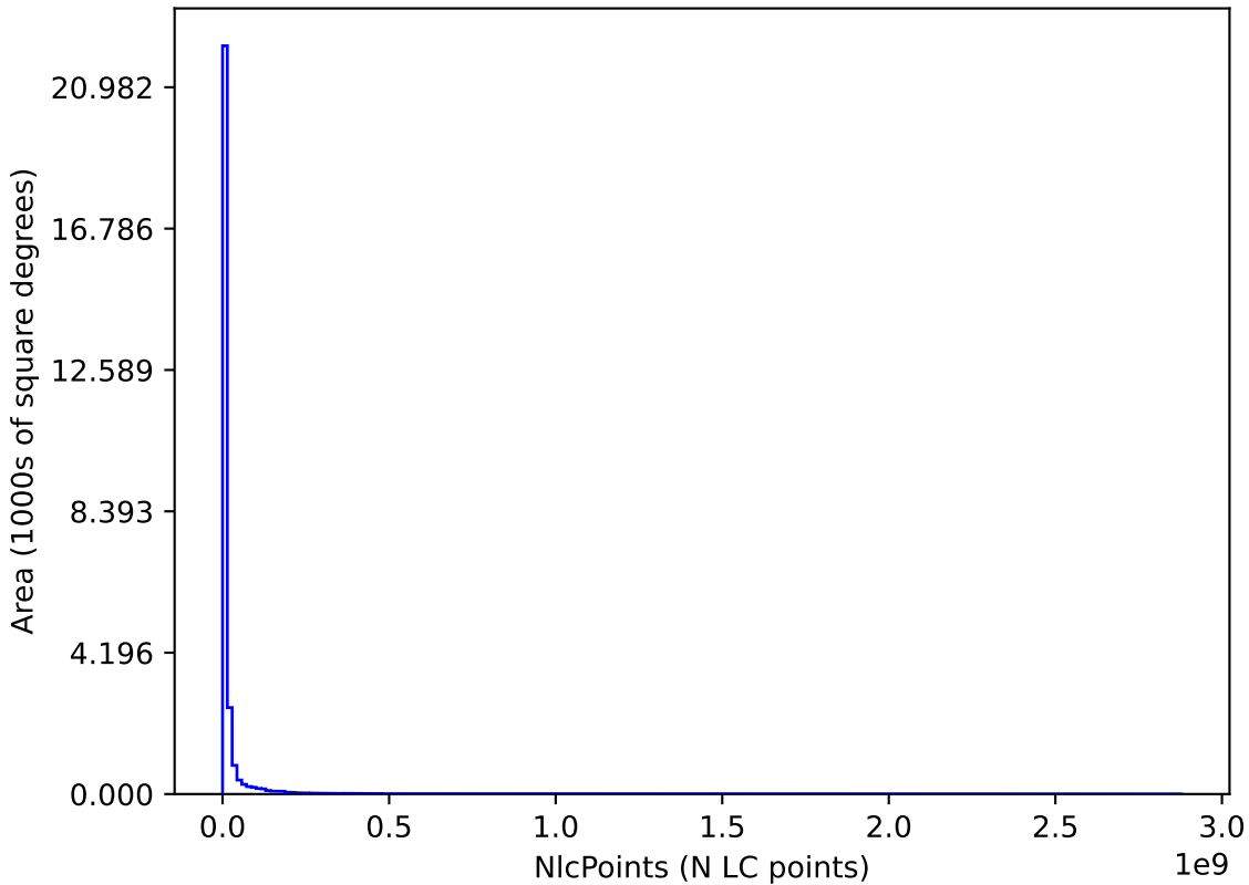
internal_u_expt60_nscale0.9v3.4_10yrs : NlcPoints
