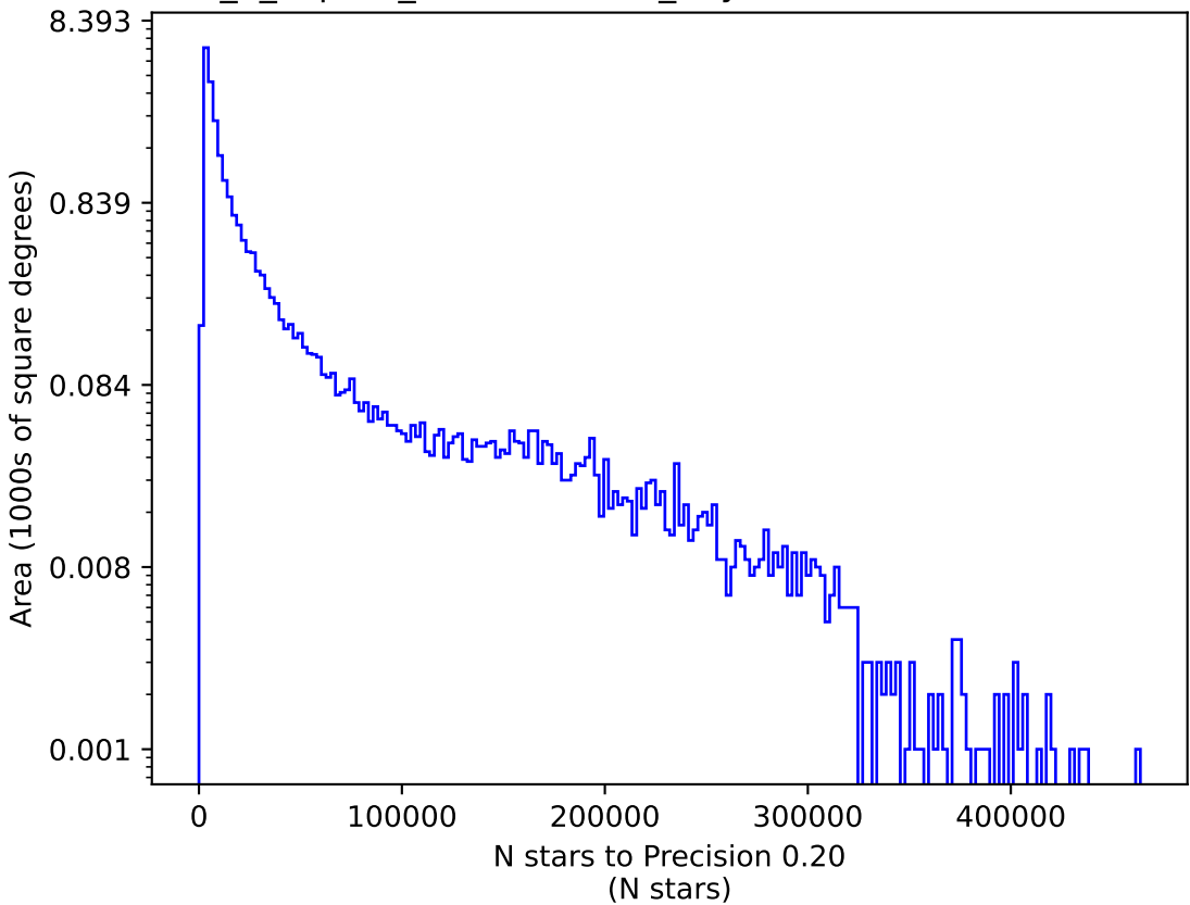
internal_u_expt60_nscale0.9v3.4_10yrs u: N stars to Precision 0.20
