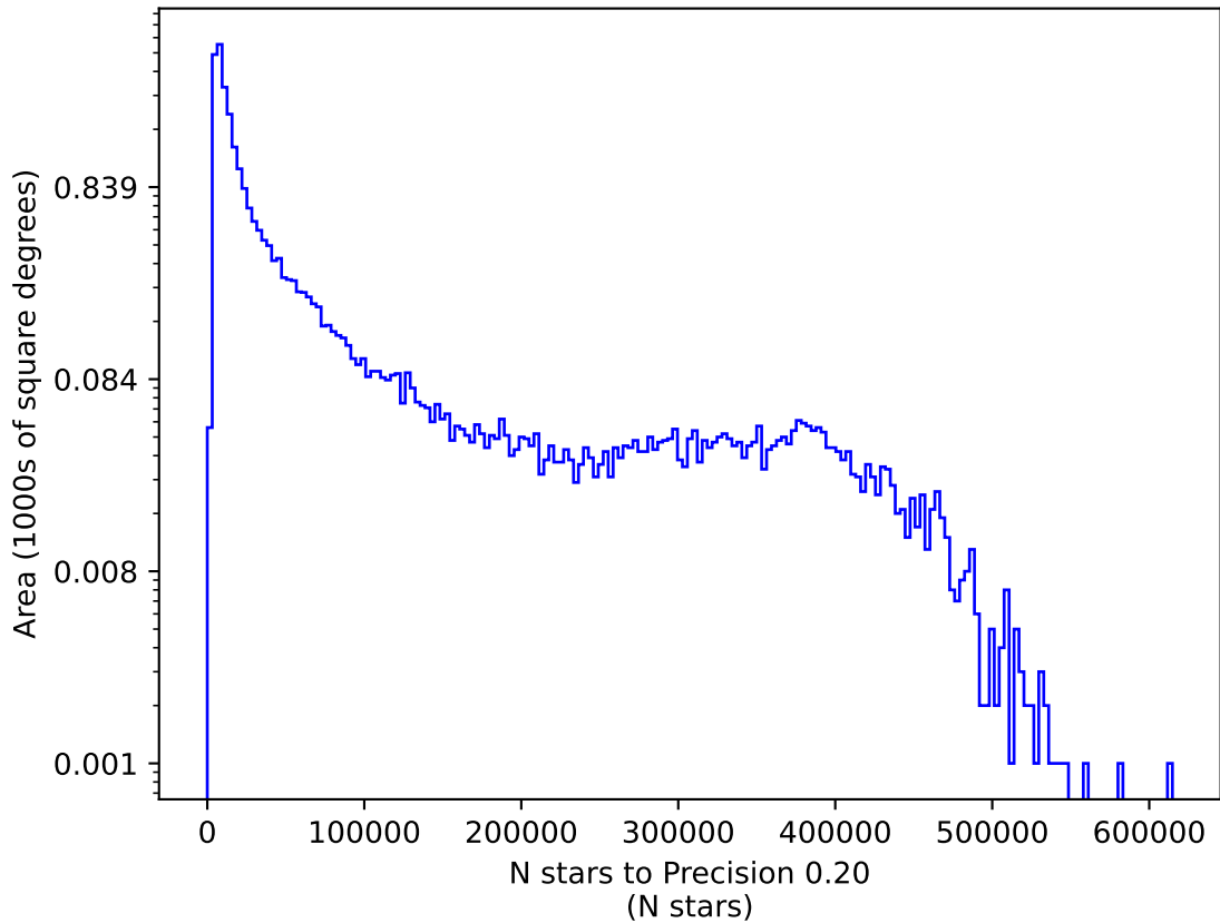
internal_u_expt60_nscale0.9v3.4_10yrs g: N stars to Precision 0.20
