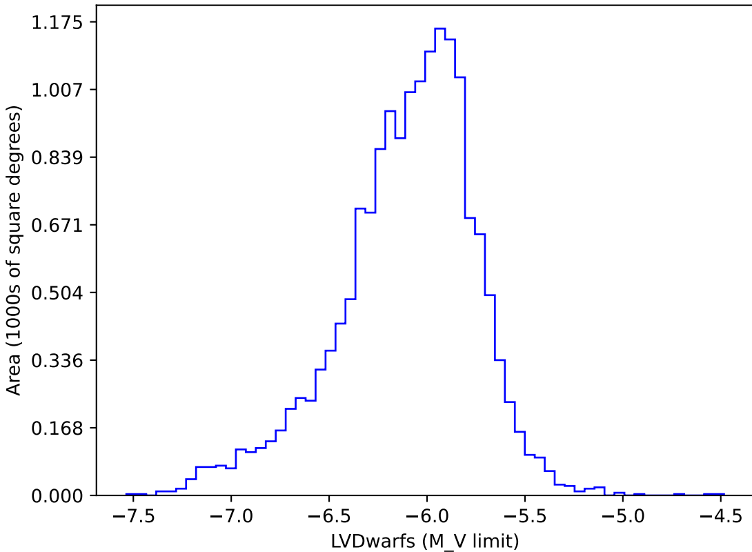
internal_u_expt60_nscale0.9v3.4_10yrs gi: LVDwarfs
