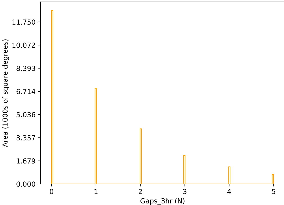
internal_u_expt60_nscale0.9v3.4_10yrs r band: Gaps_3hr
