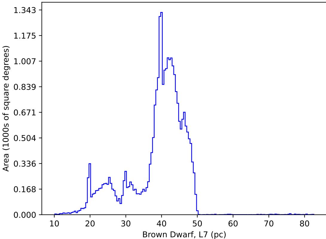
internal_u_expt60_nscale0.9v3.4_10yrs : Brown Dwarf, L7
