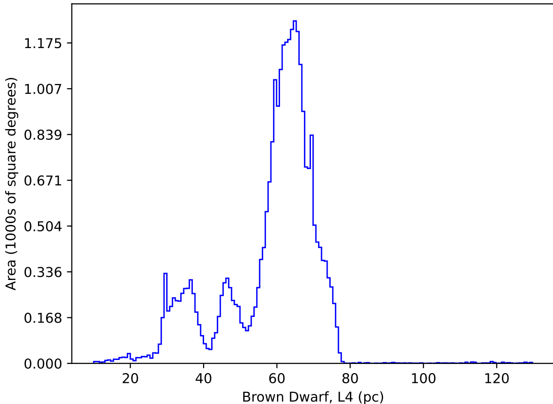
internal_u_expt60_nscale0.9v3.4_10yrs : Brown Dwarf, L4
