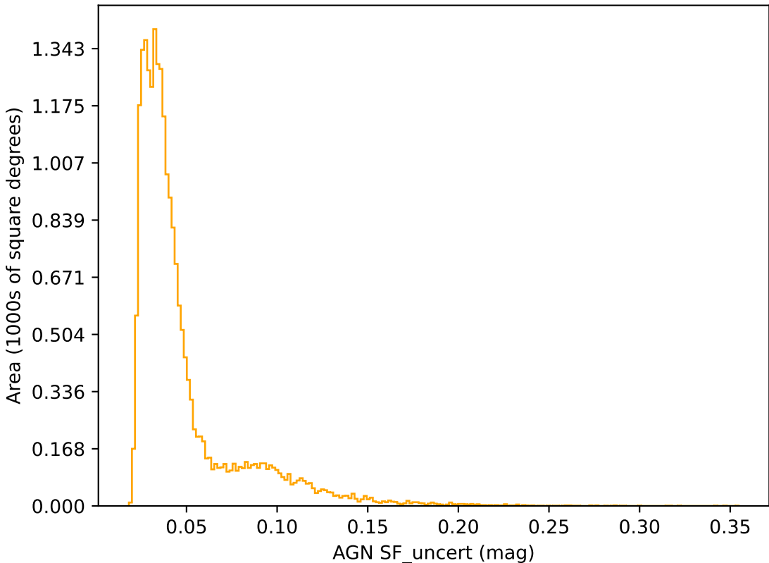
internal_u_expt60_nscale0.9v3.4_10yrs r band: AGN SF_uncert
