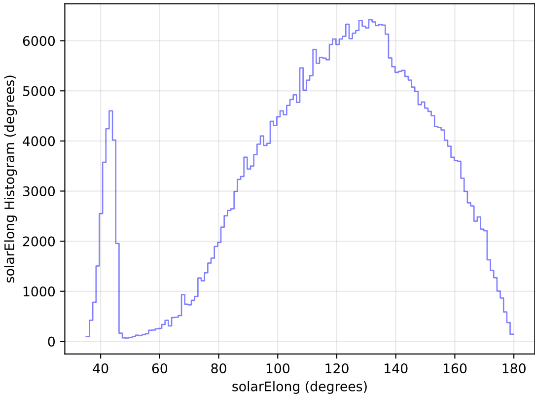
internal_u_expt60_nscale0.9v3.4_10yrs WFD z band: solarElong Histogram
